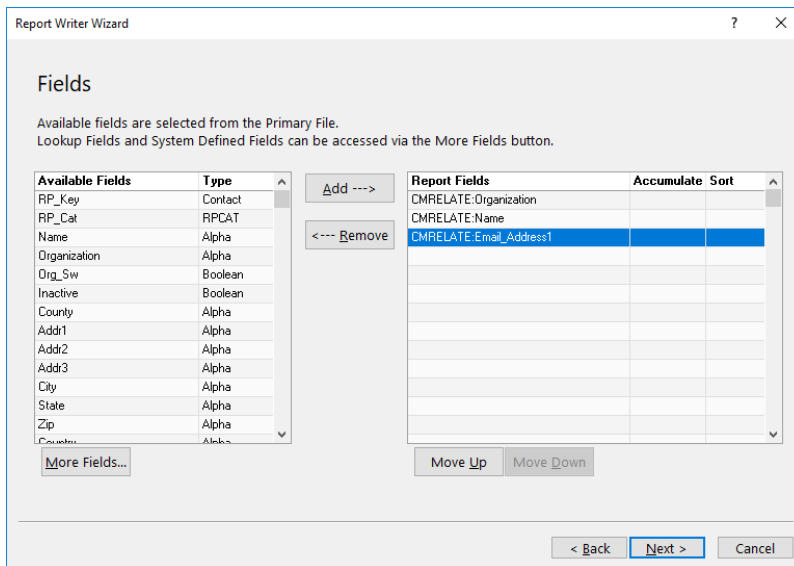
Figure 9, Report Writer Wizard - Fields panel
