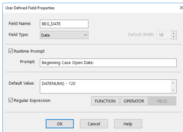
Figure 14, User Defined Field Properties window
