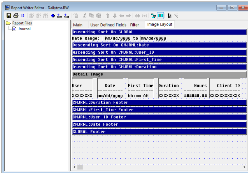
Figure 17, Report Writer Editor - Image Layout tab
