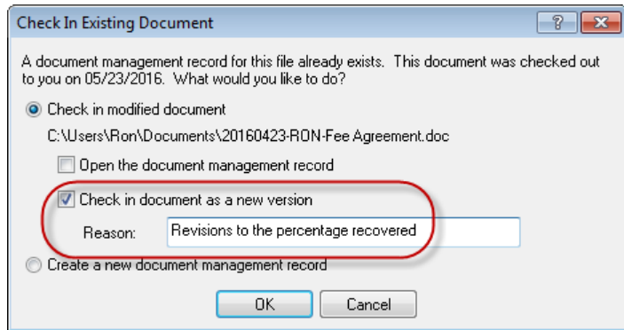
Figure 33, Check In Existing Document window
